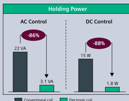
Typical Holding Power data comparison
